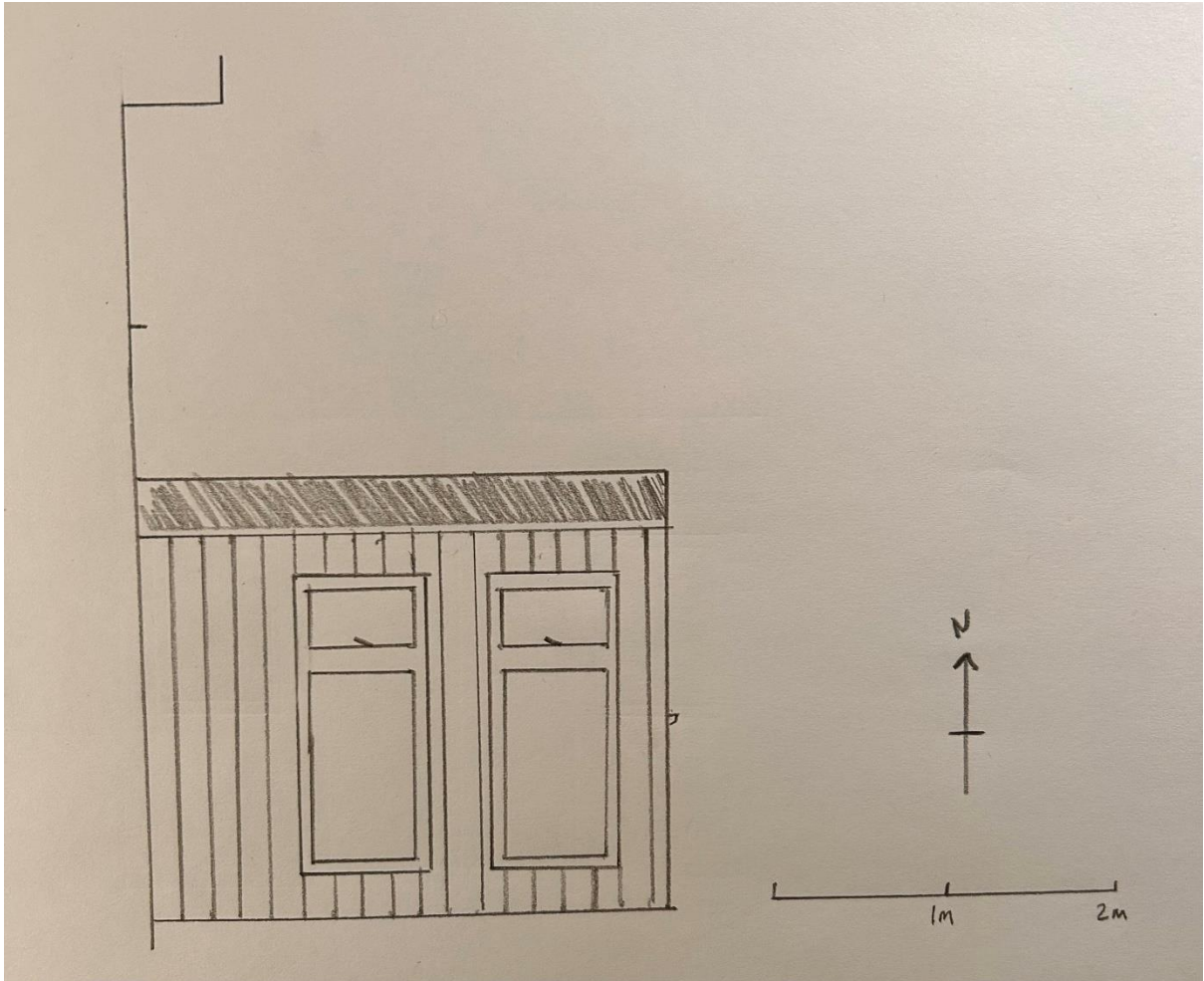
Side Elevation
