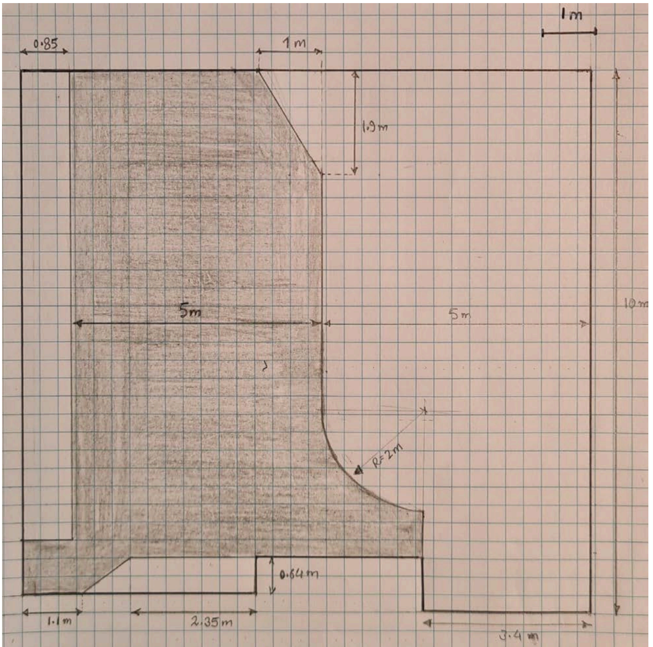
Figure3: Proposed layout for the driveway, the greyed out are is the surface that will be paved.
