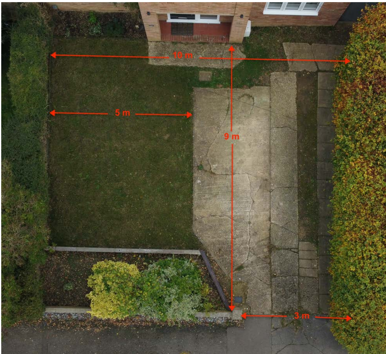
Figure 1: Photograph of the existing drive way with dimensions
